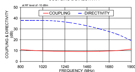
ZADC-10-17W COUPLING & DIRECTIVITY
