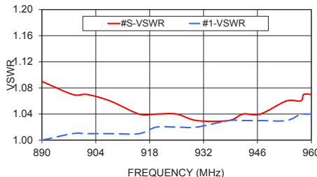
ZC16PD-960-S+ VSWR
