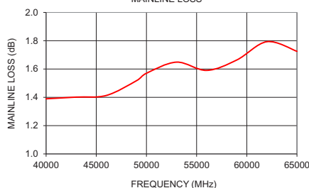
ZCDC10-E40653+ MAINLINE LOSS
