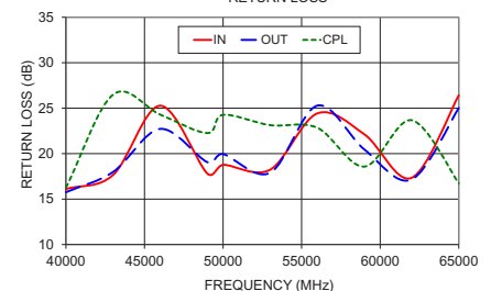
ZCDC10-E40653+ RETURN LOSS
