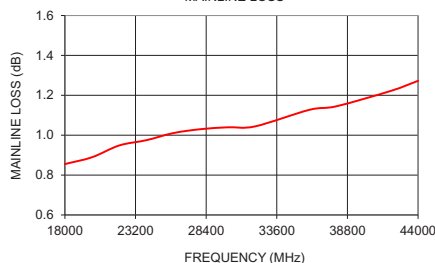
ZCDC10-V18443+ MAINLINE LOSS
