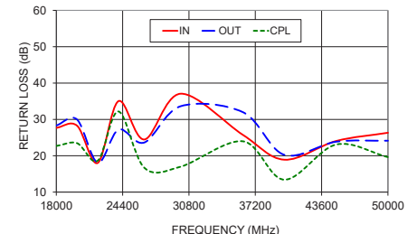
ZCDC10-V1854+ RETURN LOSS
