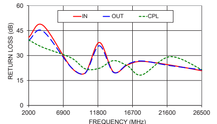
ZCDC16-02263-S+ RETURN LOSS
