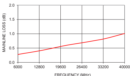
ZCDC20-K0644-S+ MAINLINE LOSS
