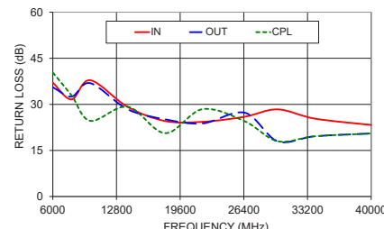
ZCDC20-K0644-S+ RETURN LOSS
