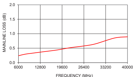
ZCDC30-K0644-S+ MAINLINE LOSS
