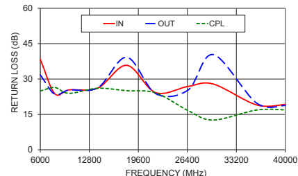
ZCDC30-K0644-S+ RETURN LOSS
