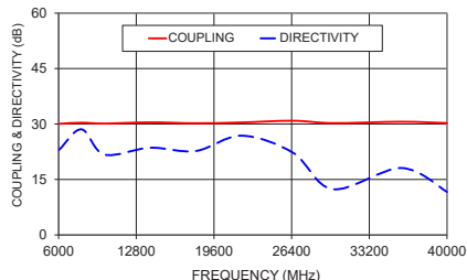
ZCDC30-K0644-S+ COUPLING & DIRECTIVITY
