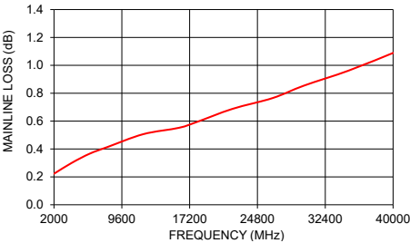
ZDDC20-K0244+ MAINLINE LOSS
