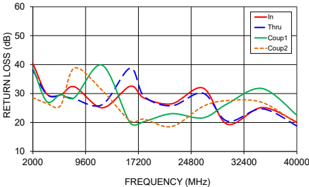
ZDDC20-K0244+ RETURN LOSS
