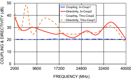
ZDDC20-K0244+ COUPLING & DIRECTIVITY
