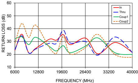
ZDDC20-K0644+ RETURN LOSS
