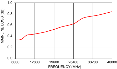
ZDDC20-K0644+ MAINLINE LOSS
