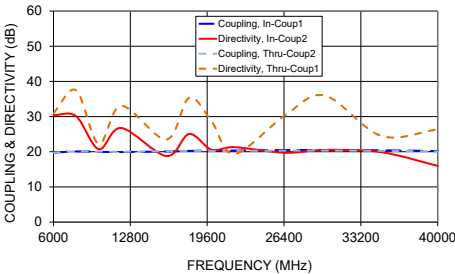
ZDDC20-K0644+ COUPLING & DIRECTIVITY
