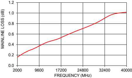
ZDDC30-K0244+ MAINLINE LOSS
