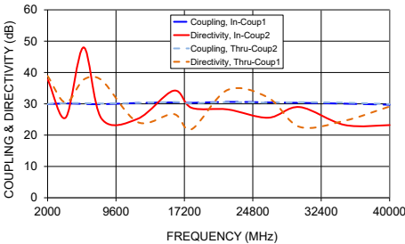
ZDDC30-K0244+ COUPLING & DIRECTIVITY
