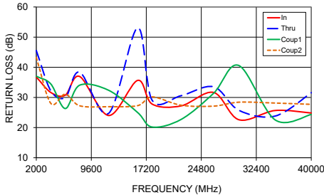
ZDDC30-K0244+ RETURN LOSS
