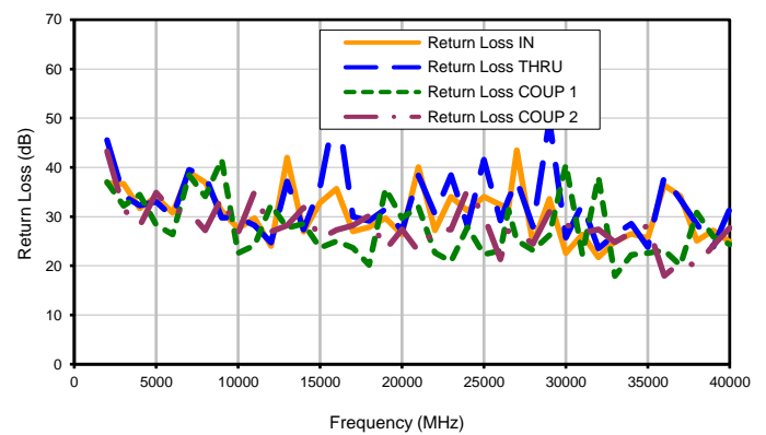
Return Loss
