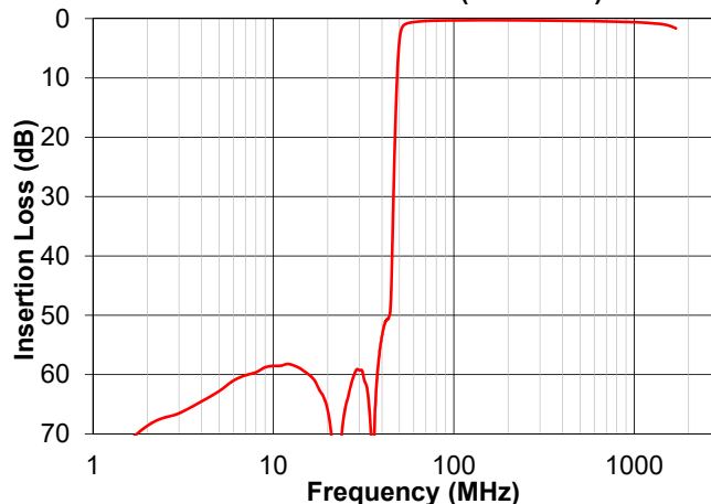
ZDPL-4254-75-F+ HIGH PASS PORT INSERTION LOSS ( P_{in}=0\text{dBm} )
