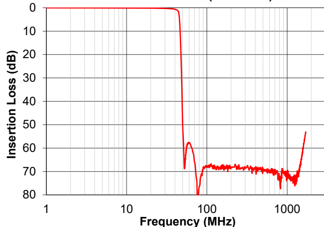
ZDPL-4254-75-F+ LOW PASS PORT INSERTION LOSS ( P_{in}=0\text{dBm} )
