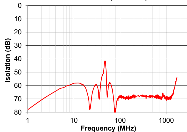
ZDPL-4254-75-F+ CROSS OVER ISOLATION ( P_{in}=0\text{dBm} )
