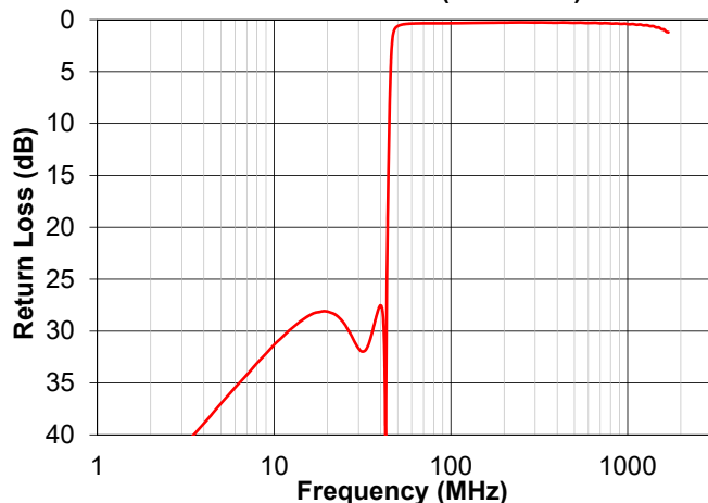
ZDPL-4254-75-F+ COMMON PORT RETURN LOSS ( P_{in}=0\text{dBm} )
