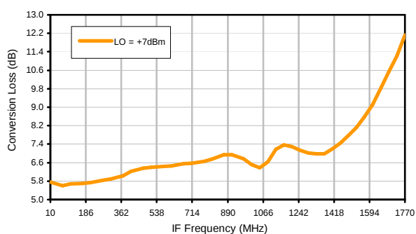
Conversion Loss vs. IF @ RF=2160.1001MHz
