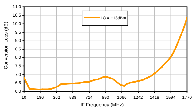
Conversion Loss vs. IF @ RF=2160.1MHz
