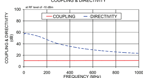
ZFDC-10-21 COUPLING & DIRECTIVITY
