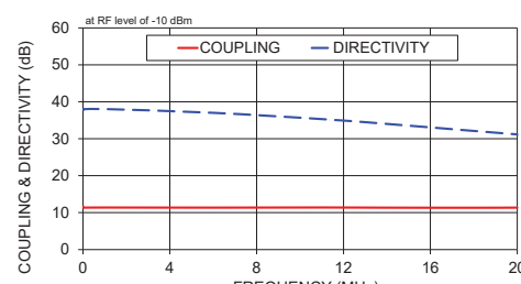
ZFDC-10-6-S+ COUPLING & DIRECTIVITY
