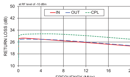
ZFDC-10-6-S+ RETURN LOSS
