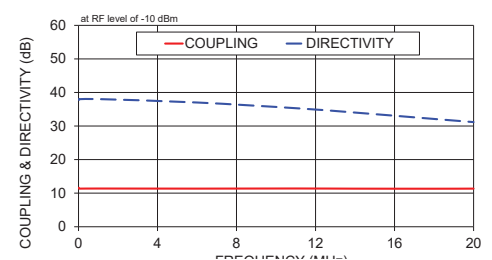
ZFDC-10-6-S+ COUPLING & DIRECTIVITY
