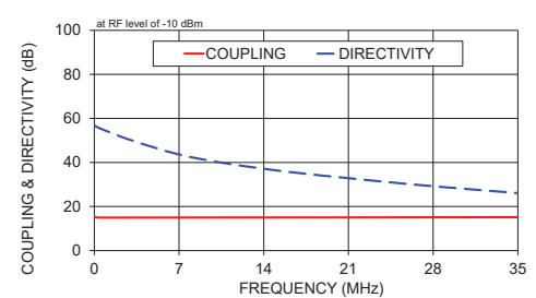
ZFDC-15-6-S+ COUPLING & DIRECTIVITY
