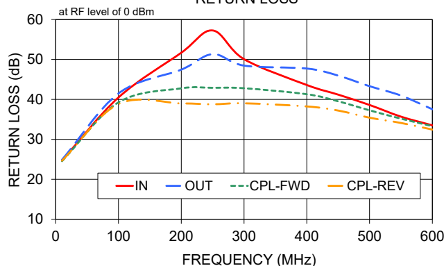
ZFDC20-62HP-S+ RETURN LOSS
