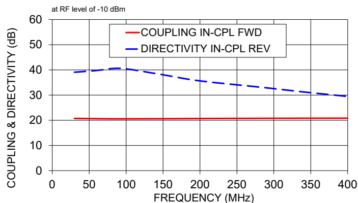
ZFDC-20-1H-S+ COUPLING & DIRECTIVITY
