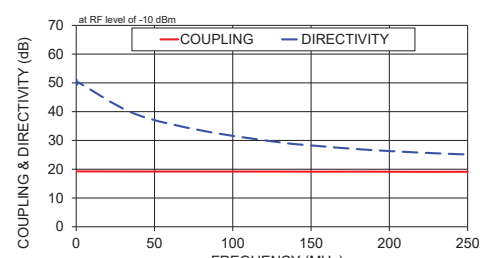
ZFDC-20-3-S+ COUPLING & DIRECTIVITY
