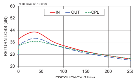
ZFDC-20-3-S+ RETURN LOSS
