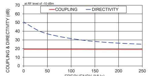
ZFDC-20-3-S+ COUPLING & DIRECTIVITY
