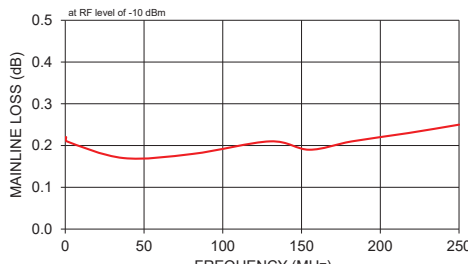
ZFDC-20-3-S+ MAINLINE LOSS
