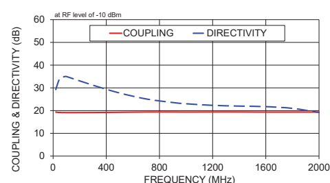
ZFDC-20-50-S+ COUPLING & DIRECTIVITY
