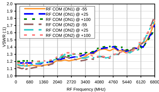
VSWR @ VDD=+5V over Temperature RF COM (ON1) & RF COM (ON2)
