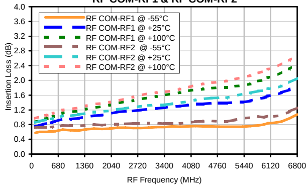
Insertion Loss @ VDD=+5V over Temperature RF COM-RF1 & RF COM-RF2
