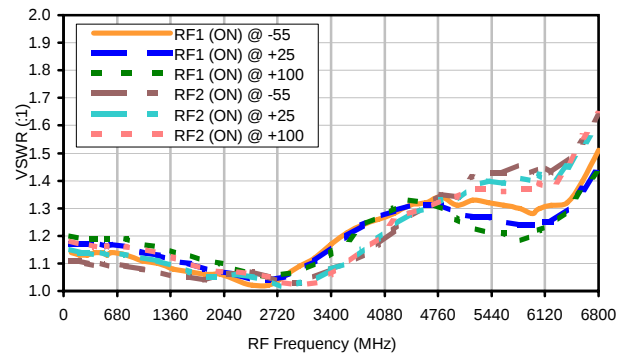
VSWR @ VDD=+5V over Temperature RF1(ON) & RF2 (ON)
