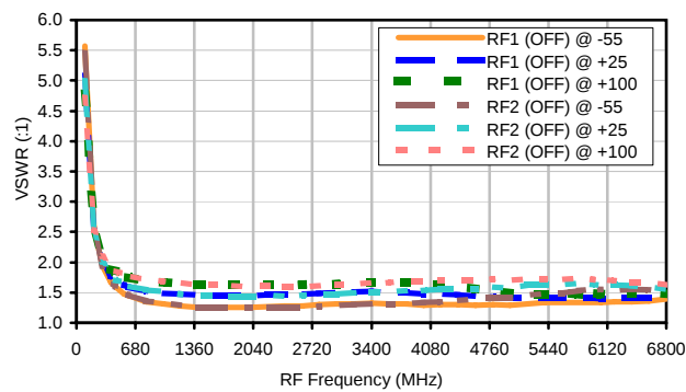
VSWR @ VDD=+5V over Temperature RF1(OFF) & RF2 (OFF)
