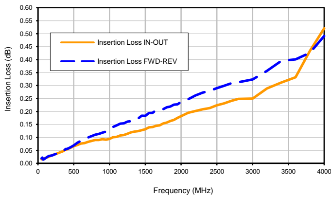
Insertion Loss
