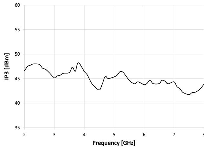
IP3 vs. Frequency
