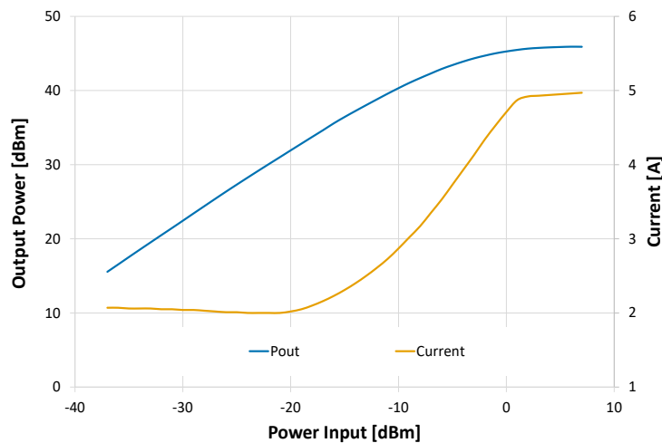
Power Out & Current vs. Power In @ 5000 MHz
