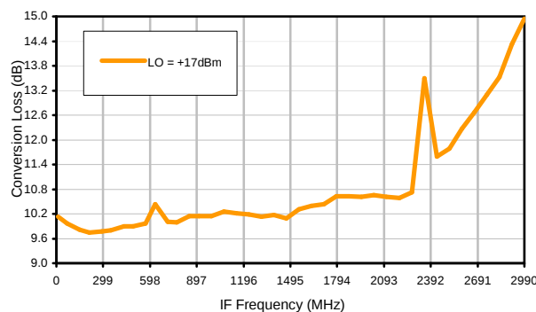
Conversion Loss vs. IF @ RF=3000.1001MHz
