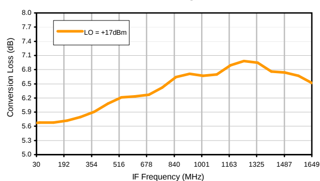
Conversion Loss vs. IF @ RF=7010.1MHz
