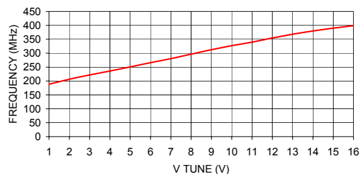
ZOS-400 FREQUENCY vs. TUNING VOLTAGE
