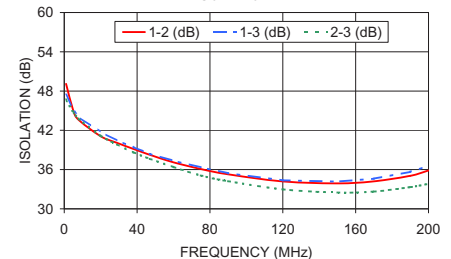
ZSC-3-1 ISOLATION
