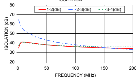
ZSC-4-1-75+ ISOLATION
