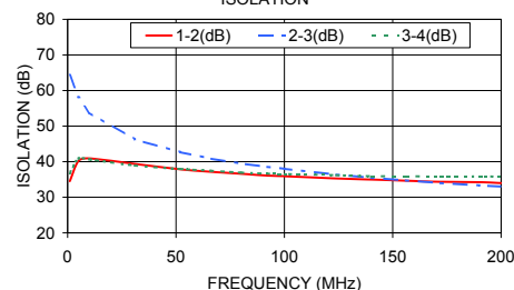
ZSC-4-1-75+ ISOLATION
