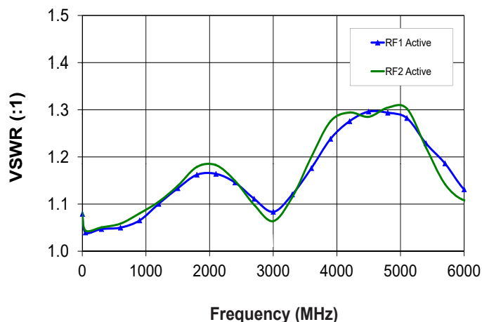
VSWR @ Active Ports RF1/2
