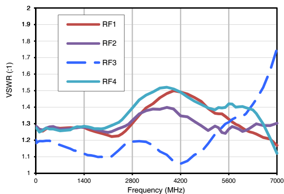
Off (terminated) State VSWR Temperature = -40°C
