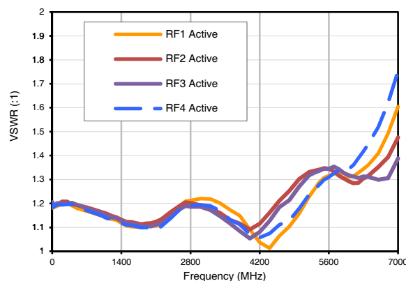
VSWR (RF1, RF2, RF3, RF4) Temperature = -40°C
