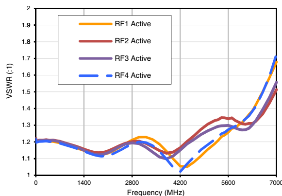
VSWR (RF1, RF2, RF3, RF4) Temperature = +25°C
