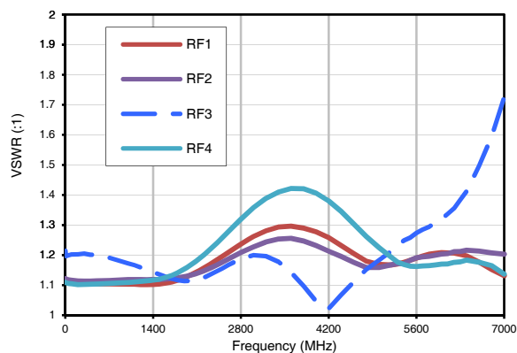
Off (terminated) State VSWR Temperature = +25°C
