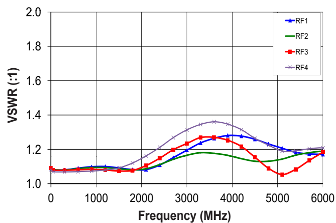
VSWR terminated port vs. Frequency
