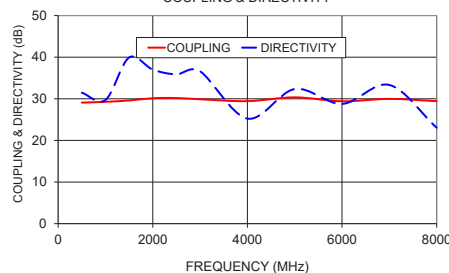
ZUDC30-83-S+ COUPLING & DIRECTIVITY
