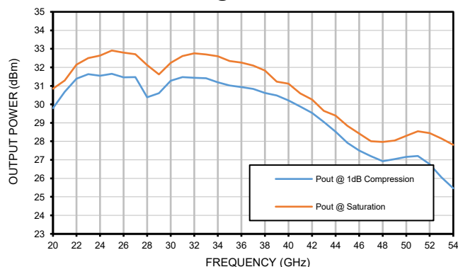
OUTPUT POWER @MINIMUM ATTENUATION
