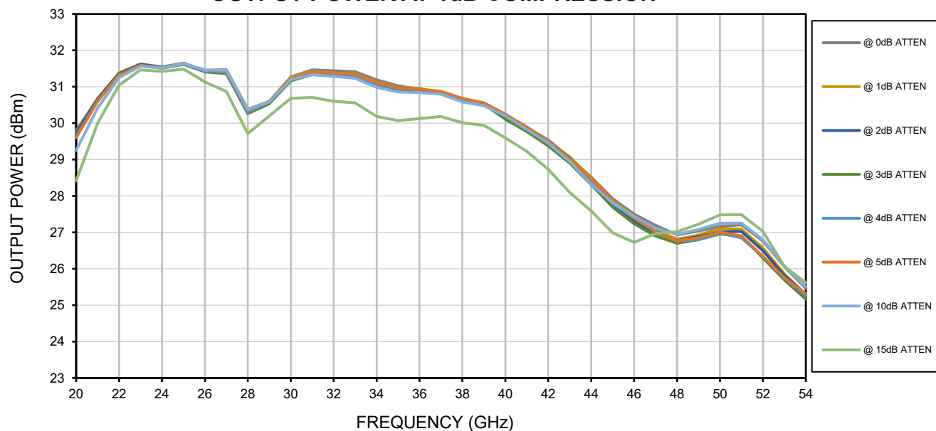
OUTPUT POWER AT 1dB COMPRESSION
