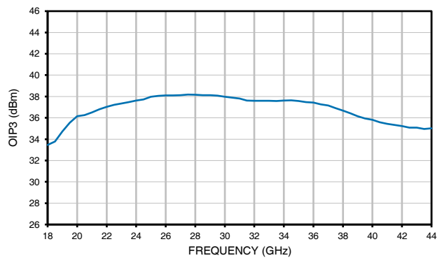
OUTPUT IP3
