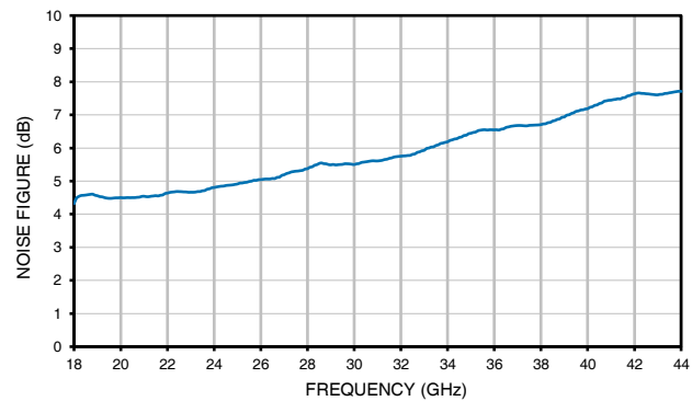
NOISE FIGURE
