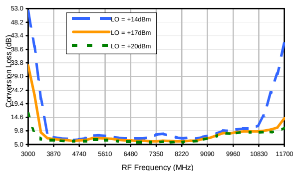
Conversion Loss vs. LO @ RF=6850MHz
