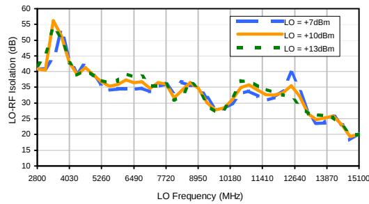
LO-IF Isolation
