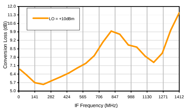
Conversion Loss vs. IF @ RF=4210.1001MHz
