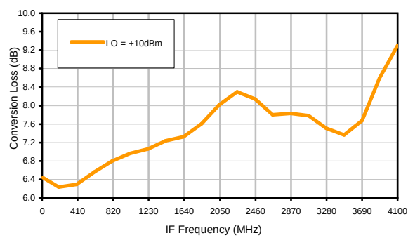
Conversion Loss vs. IF @ RF=15010.099MHz
