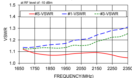
ZX10-4-24-S+ VSWR
