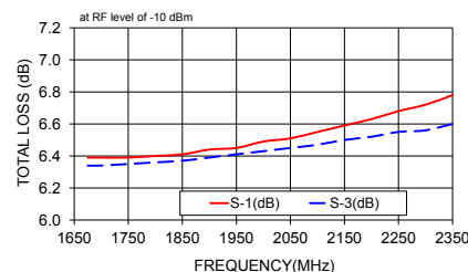
ZX10-4-24-S+ TOTAL LOSS
