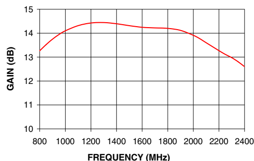
GAIN
