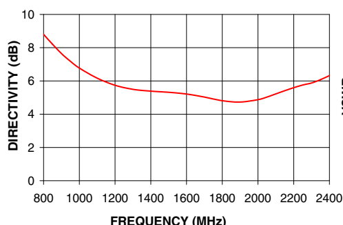
DIRECTIVITY
