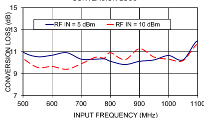
ZX90-2-11-S+ CONVERSION LOSS
