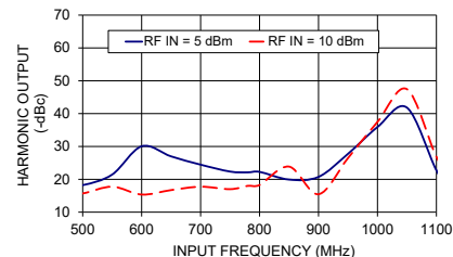
ZX90-2-11-S+ HARMONIC OUTPUT F4
