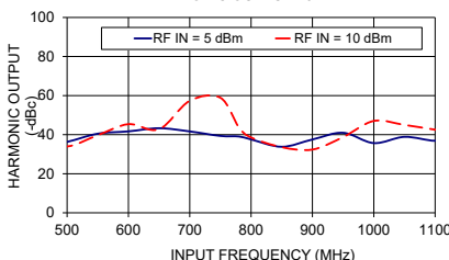
ZX90-2-11-S+ HARMONIC OUTPUT F3
