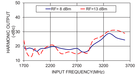
ZX90-2-36-S+ HARMONIC OUTPUT F4
