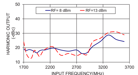
ZX90-2-36-S+ HARMONIC OUTPUT F4
