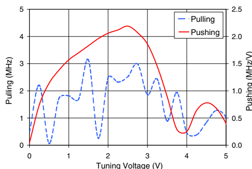
ZX95-2650A-S+ Frequency Pulling & Pushing (Vcc ± 5%)
