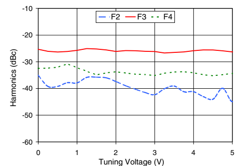
ZX95-2650A-S+ Harmonics Level
