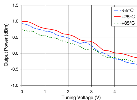
ZX95-2650A-S+ Power Output
