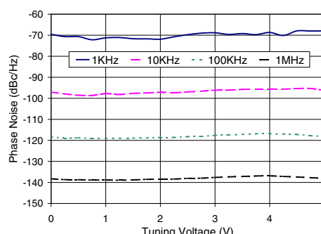
ZX95-2650A-S+ Phase Noise Vs. Tuning Voltage
