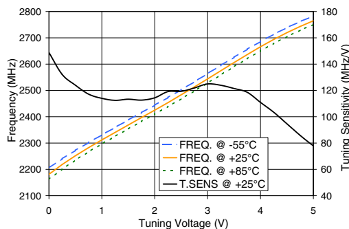
ZX95-2650A-S+ Frequency and Tuning Sensitivity
