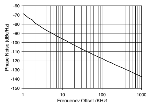
ZX95-2650A-S+ Phase Noise
