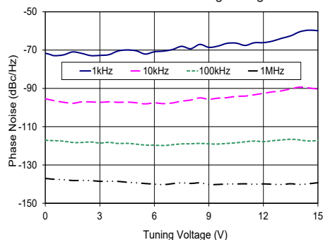
ZX95-4650-S+ Phase Noise Vs. Tuning Voltage
