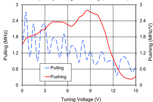
ZX95-4650-S+ Frequency Pulling & Pushing (Vcc ± 5%)
