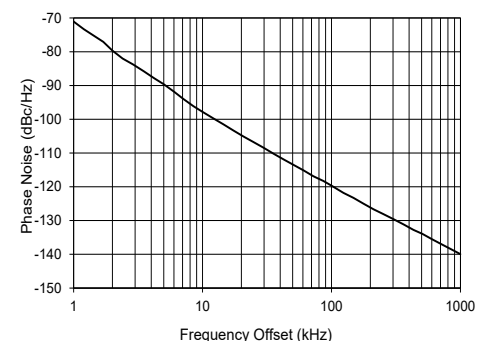
ZX95-4650-S+ Phase Noise
