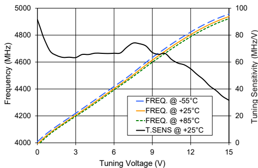
ZX95-4650-S+ Frequency and Tuning Sensitivity
