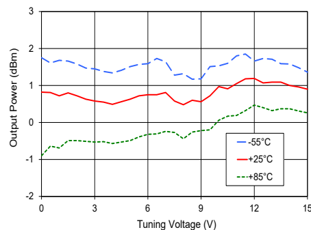
ZX95-4650-S+ Power Output
