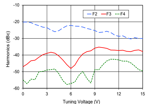
ZX95-4650-S+ Harmonics Level
