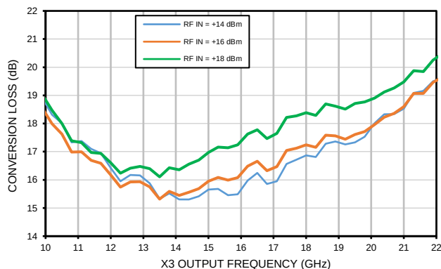
CONVERSION LOSS X3 OUTPUT
