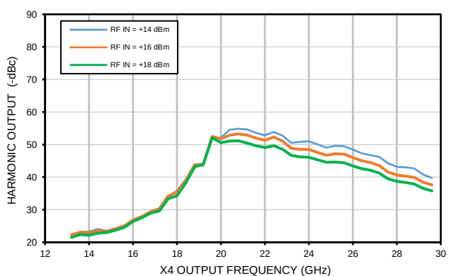
HARMONIC X4 OUTPUT
