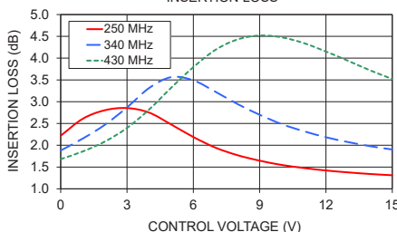
ZXPHS-431+ INSERTION LOSS
