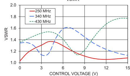
ZXPHS-431+ VSWR
