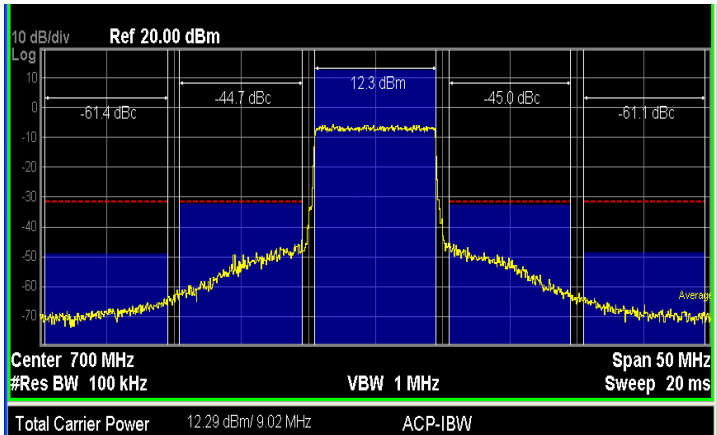
Figure 2 ACLR Plot at Output Power of +12.29 dBm
