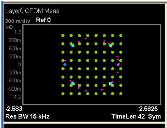
Figure 3 EVM Plot at Output Power of +12.29 dBm
